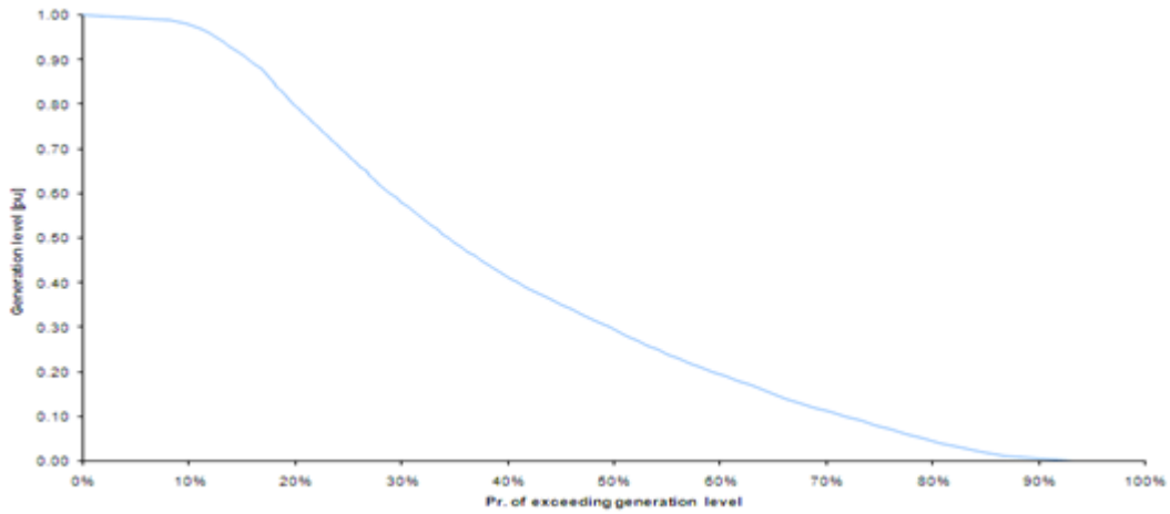
Figure 4: Generation duration curve
